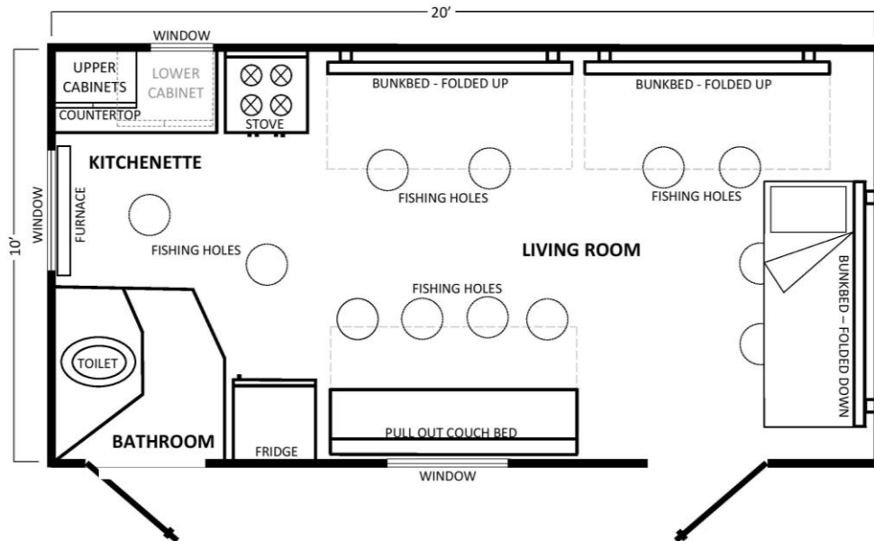
AIDEN'S ICE BUNGALOWS 20' FLOOR PLAN NOT TO SCALE
